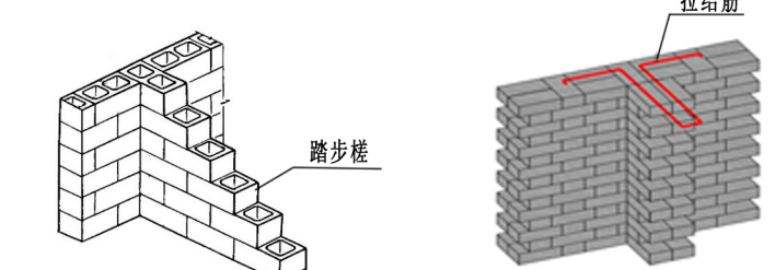
纵横墙交接处砌成踏步槎 (✓)
